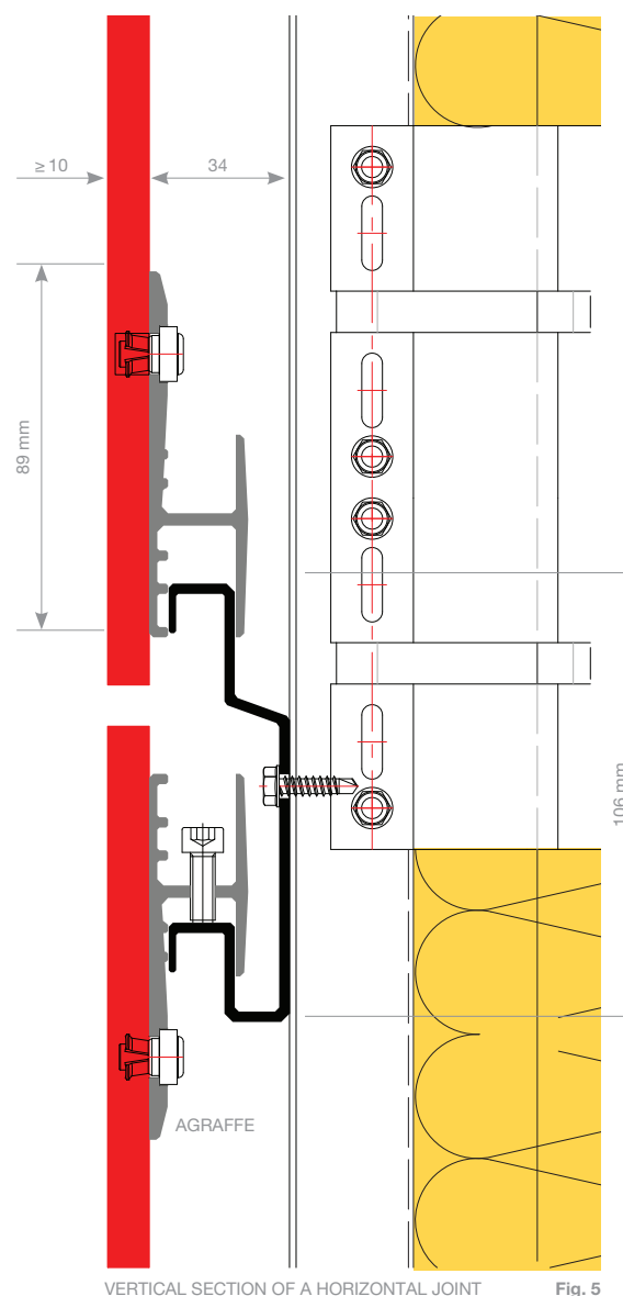
VERTICAL SECTION OF A HORIZONTAL JOINT
