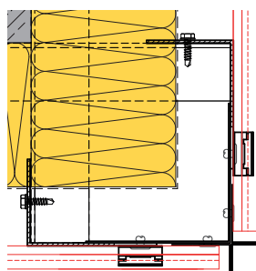
EXTERNAL CORNER A105 WITH CROSS PROFILE
