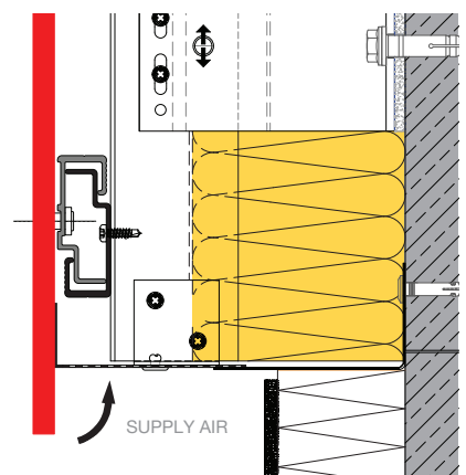
BASE CONNECTION A103
