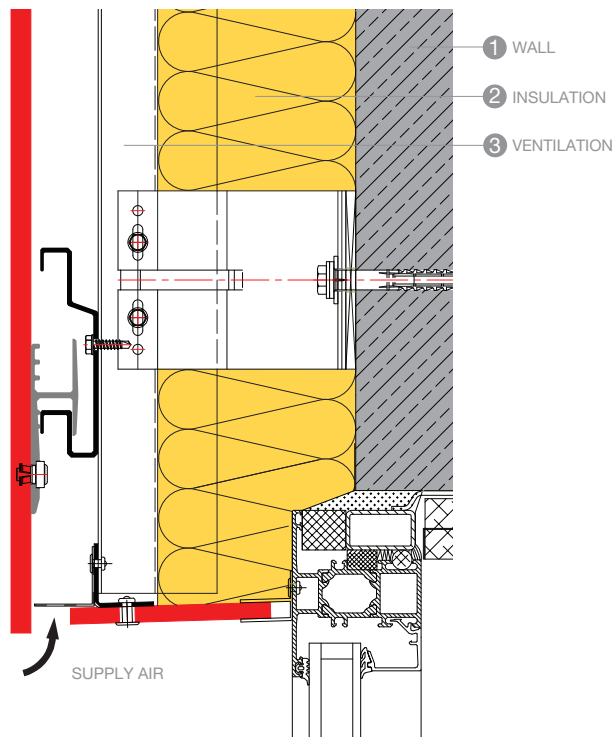
WINDOW LINTEL A101
