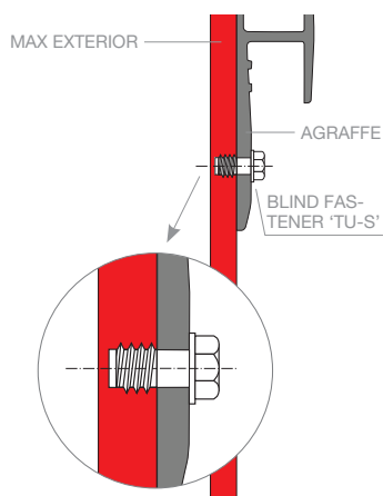
DETAIL BLIND FASTENER
