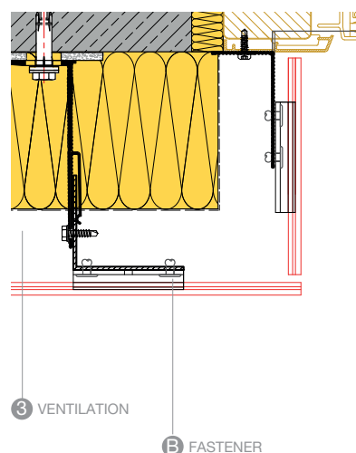
WINDOW REVEAL A104
