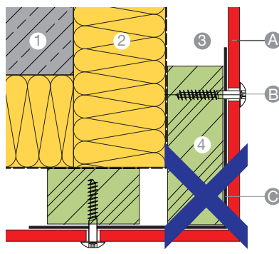
HORIZONTAL SECTION
