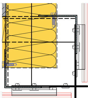
EXTERNAL CORNER A105 WITH CROSS PROFILE
