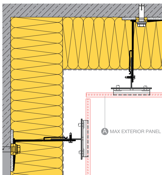
INTERNAL CORNER A106
