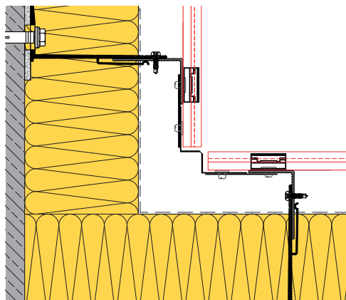
INTERNAL CORNER A106 WITH PROFILE
