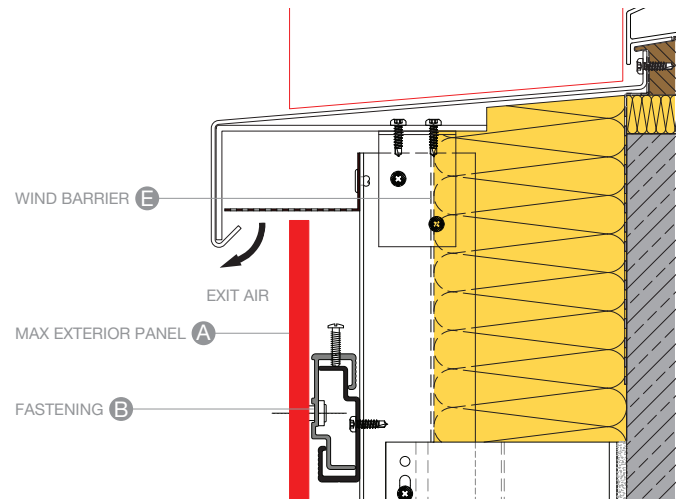
WINDOW SILL CONNECTION A102
