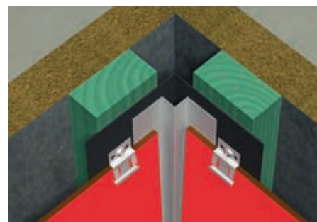
INTERNAL CORNER PROFILE
