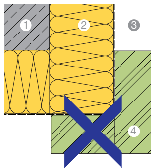
HORIZONTAL SECTION
