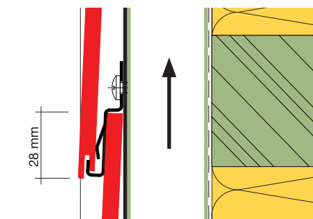
OVERLAP DIMENSION SCALEO ELEMENTS
