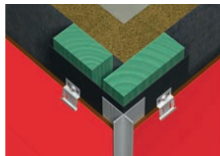
EXTERNAL CORNER WITH CROSS PROFILE
