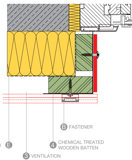
WINDOW REVEAL A104
