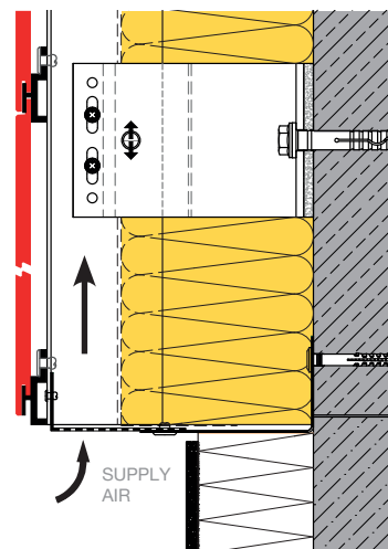
BASE CONNECTION A103
