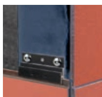
OPEN CORNER JOINT WITH EPDM PROTECTIVE TAPE Fig. 2
