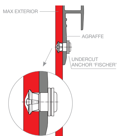
DETAIL UNDERCUT ANCHOR
