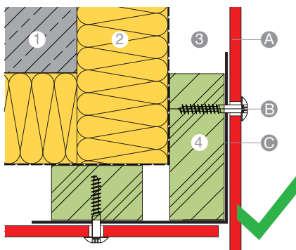
HORIZONTAL SECTION
