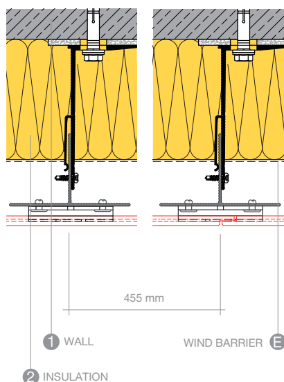
SUPPORT BETWEEN A108
