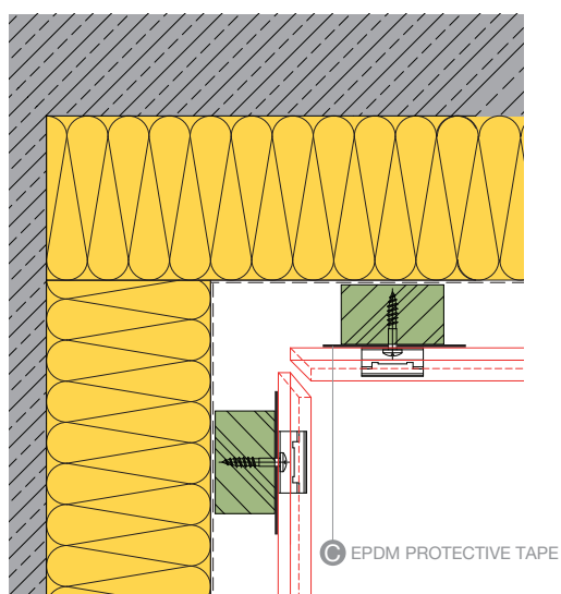
INTERNAL CORNER A106
