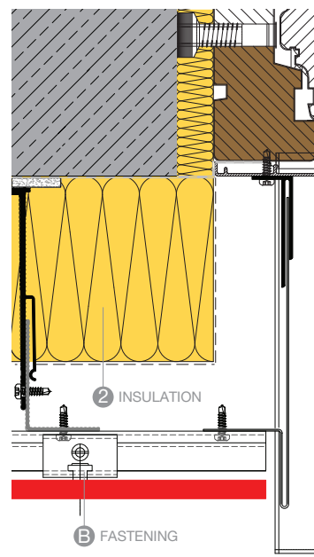
WINDOW REVEAL A104
